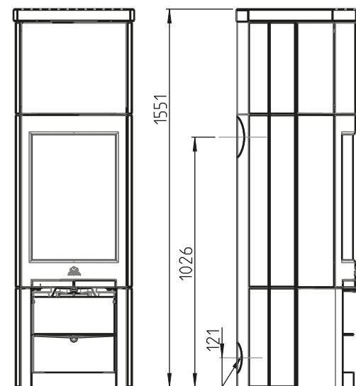
Jøtul F 367 Advance with High Top
