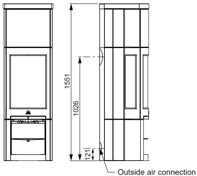
Jøtul F 377 Advance with High Top
